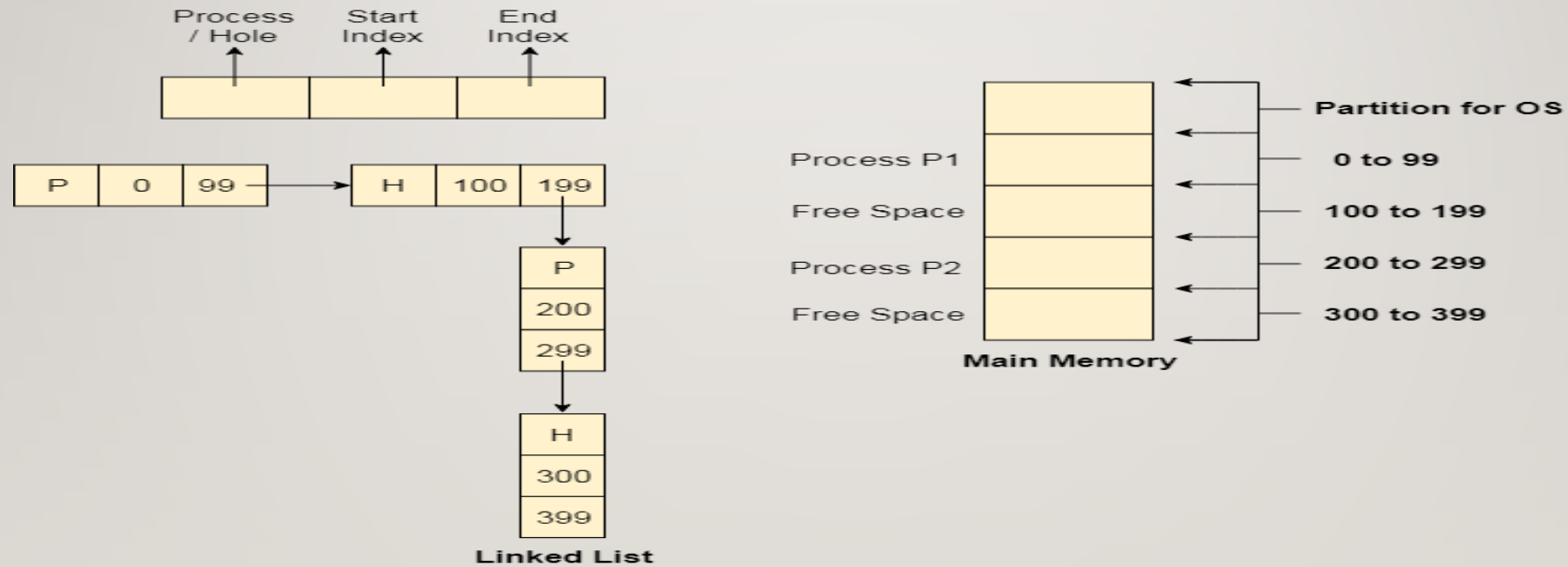
Linked List for Dynamic Partitioning
